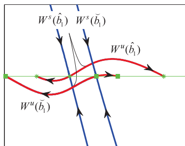
Fig. 3. Stable manifolds W^s(\hat{b}_1) , W^s(\tilde{b}_1) (indicated as blue lines) and unstable manifolds W^u(\hat{b}_1) , W^u(\tilde{b}_1) (indicated as red lines) of (\hat{b}_1, 0) and (\tilde{b}_1, 0) . (For interpretation of the references to color in this figure legend, the reader is referred to the web version of this article.)
