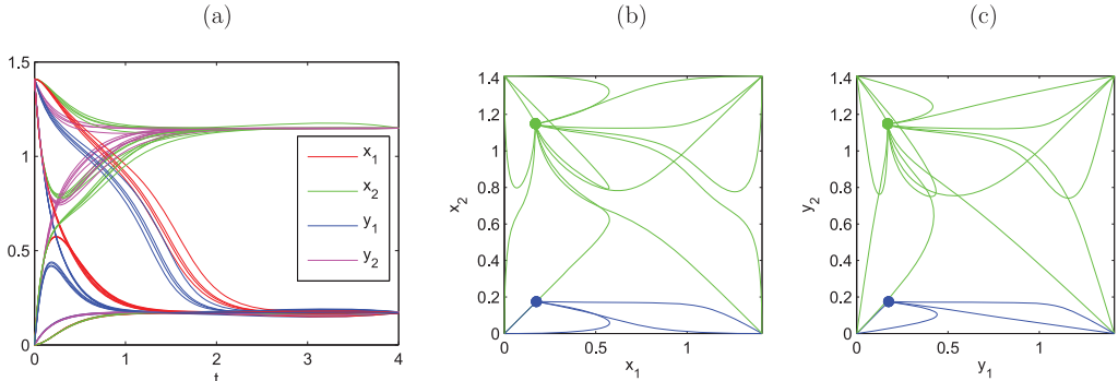
Fig. 7. ODE simulation (a) x_1, x_2, y_1, y_2 versus t , (b) the trajectories in (x_1, x_2) -plane, (c) the trajectories in (y_1, y_2) -plane. (For interpretation of the references to color, the reader is referred to the web version of this article.)
