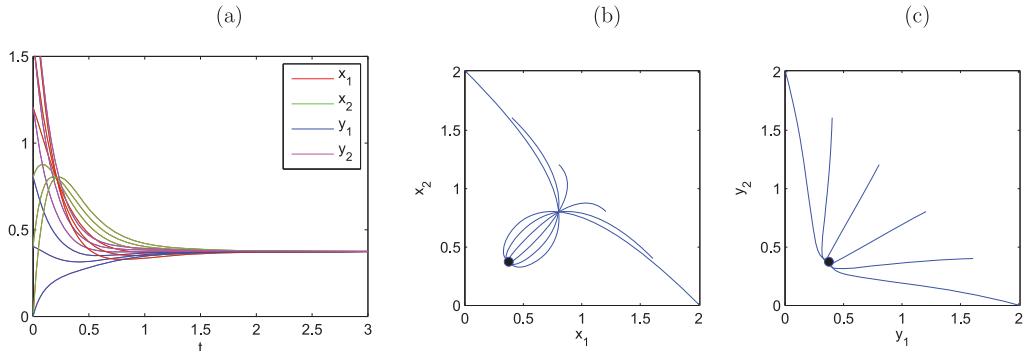
Fig. 6. ODE simulation (a) x_1, x_2, y_1, y_2 versus t , (b) the trajectories in (x_1, x_2) -plane, (c) the trajectories in (y_1, y_2) -plane.
