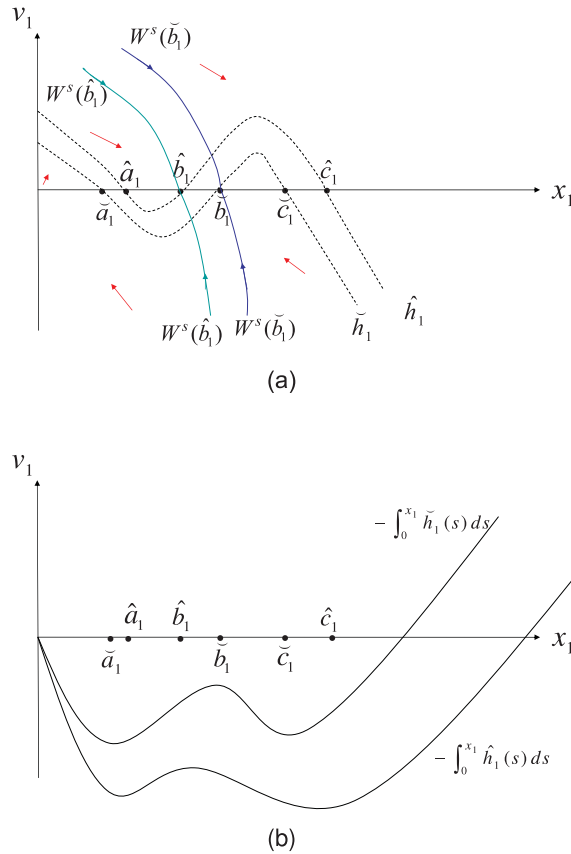
Fig. 4. (a) The vector field for (3.9)–(3.10) projected onto (x_1, v_1) -plane. (b) The graphs for -\int_0^{x_1} \hat{h}_1(s) ds and -\int_0^{x_1} \check{h}_1(s) ds .
